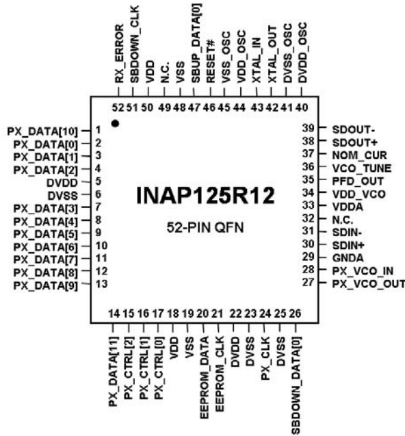
Figure 10-1: INAP125R12 pinout diagram
