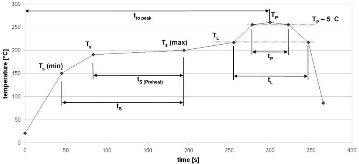
Figure 9-1: Reflow profile
