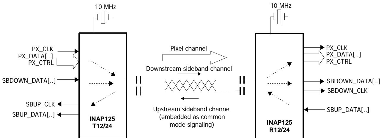
Figure 1-1: Single wire transmission channel configuration
