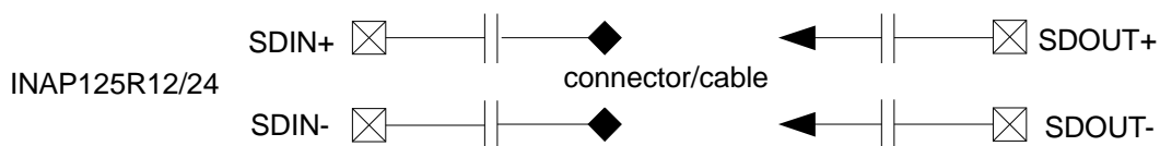
Figure 5-1: External coupling capacitors in downstream
