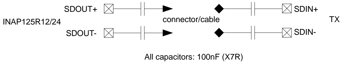
Figure 5-2: External coupling capacitors in upstream
