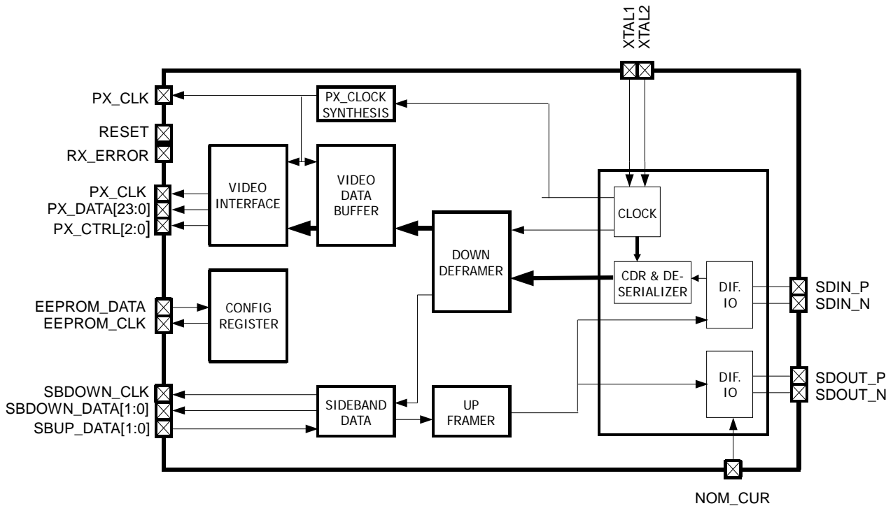
Figure 2-2: INAP125R24 Block Diagram
