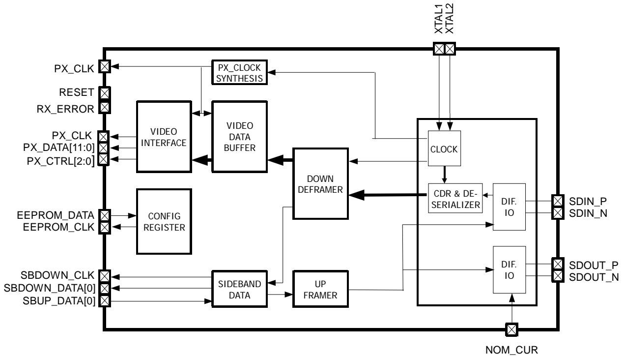
Figure 2-1: INAP125R12 Block Diagram
