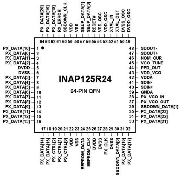
Figure 10-2: INAP125R24 pinout diagram
