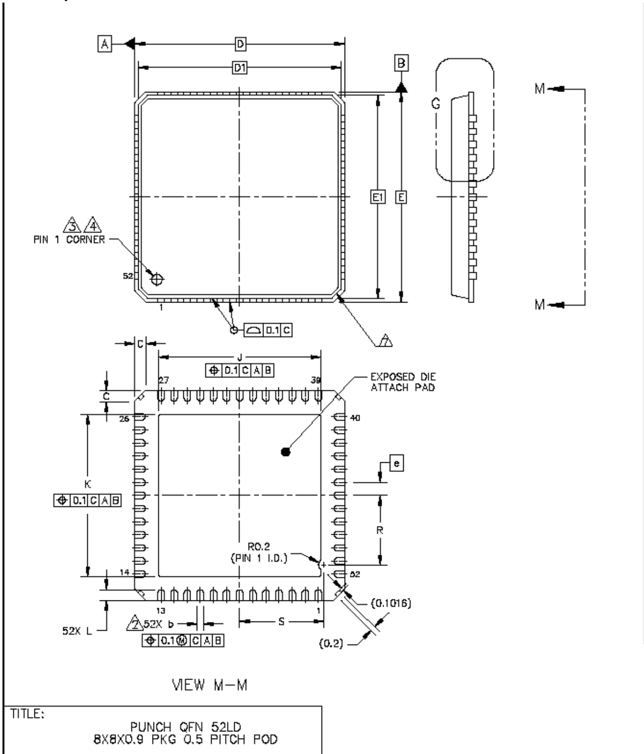
Figure 10-3: 52-pin QFN package dimensions
