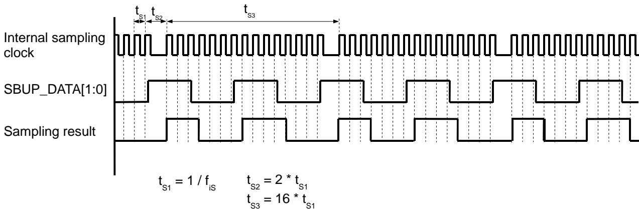
Figure 2-4: Asynchronous sampling of SBUP_DATA[1:0]
