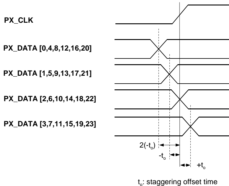
Figure 2-3: Staggered pixel interface outputs
