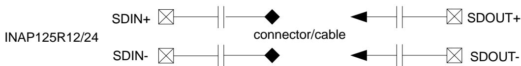
Figure 5-1: External coupling capacitors in downstream
